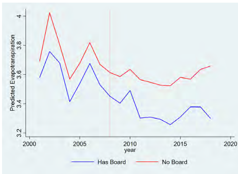
Figure V: Predicted ETa by Water Board presence and year.
