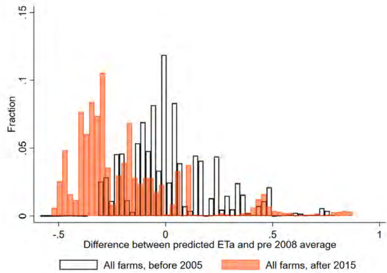
Figure IV: Predicted ETa by Water Board presence and year.
