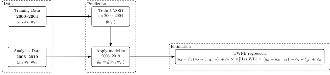
Figure XI: Diagram: construction of the Drought index.
