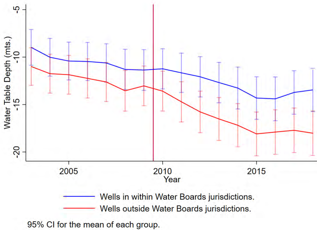
(a) Average water table depth, by Water Board presence, for monitoring stations with data at least from 1998 onwards. Negative numbers correspond to lower water table levels, indicating dryer wells.
