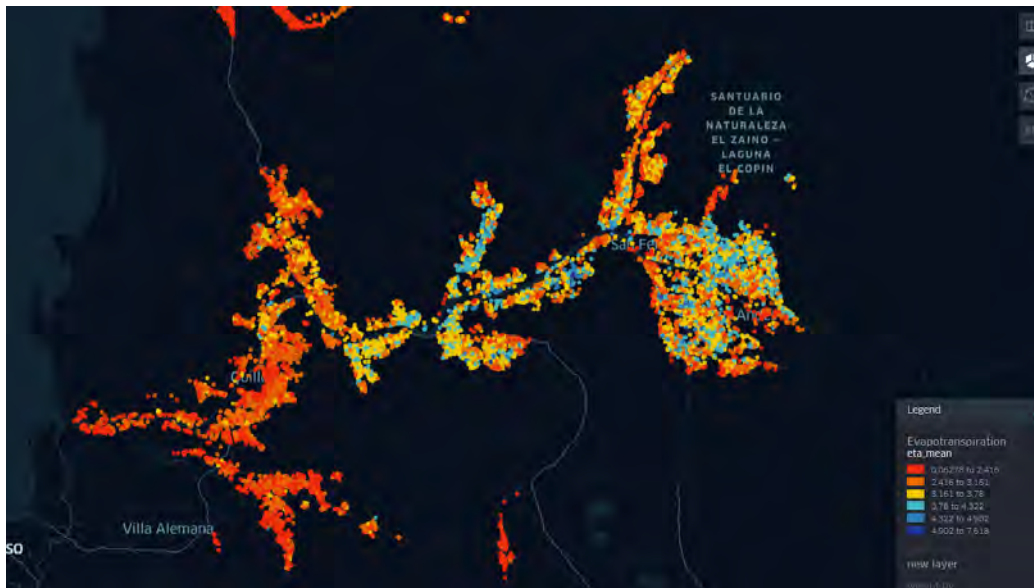
Figure III: Farm level summer evapotranspiration estimates for the Aconcagua Basin (2000-2005).
